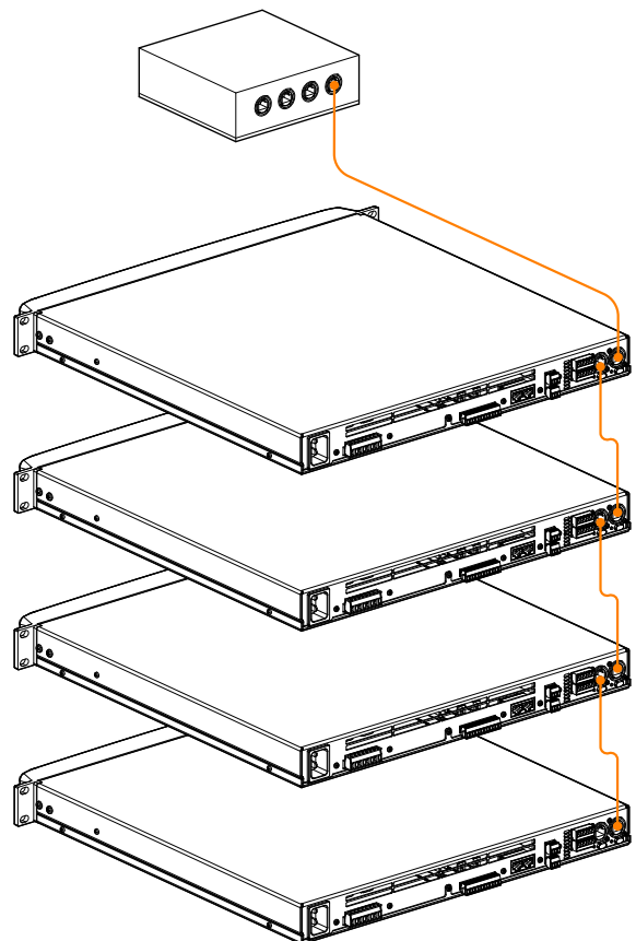
2. DAISY-CHAIN Connection
