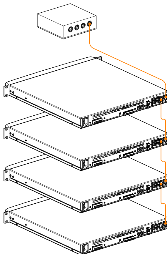
2. Connessione DAISY-CHAIN
