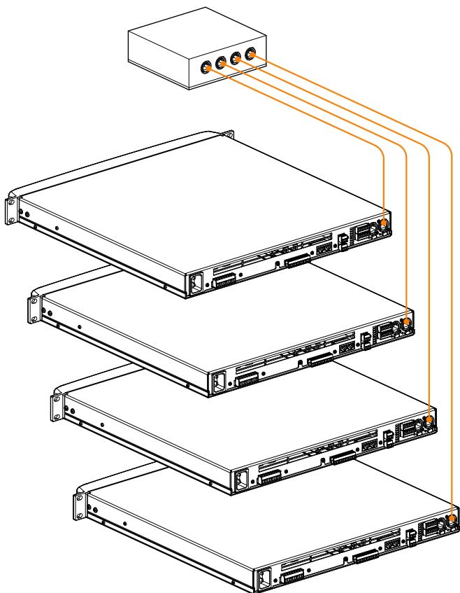
1. STAR Connection
